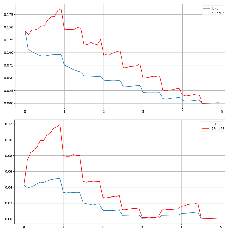
Figure 3: Expected exposure and quantile potential future exposure profiles with and without netting rules applied for a portfolio of 10 instruments
