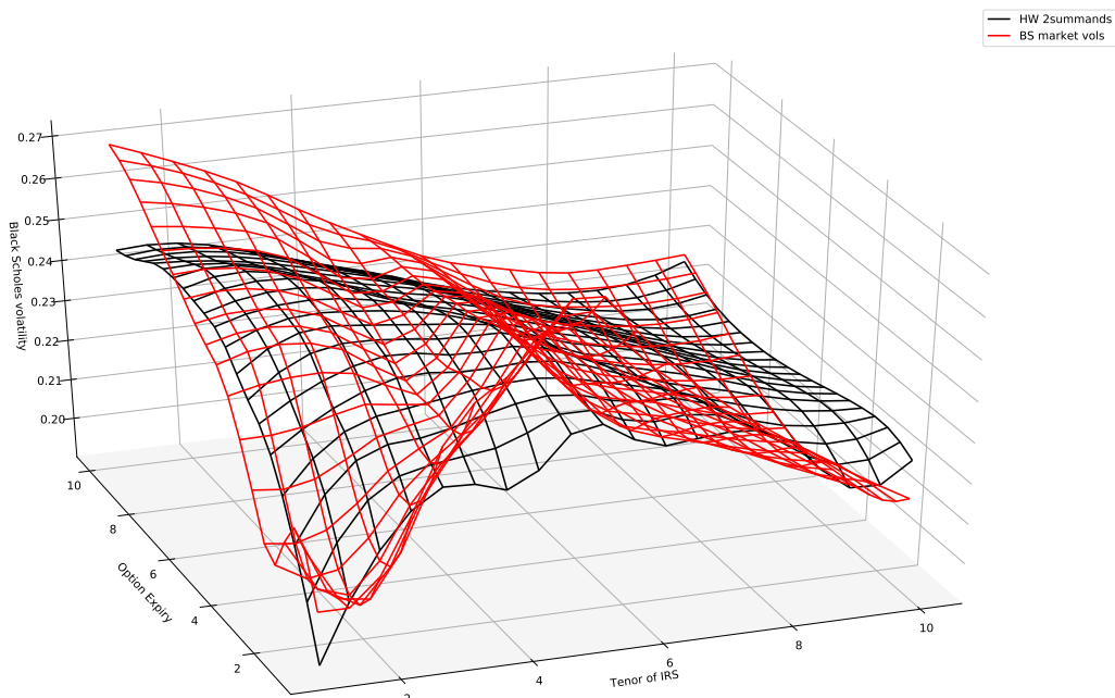
Figure 2: Market (BS) and calibrated implied volatility in Hull-White with two summands as of 20th Nov 2017
