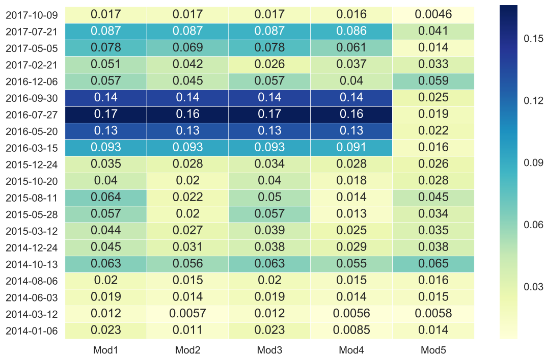
Figure 1: Objective function values for different models calibrated
