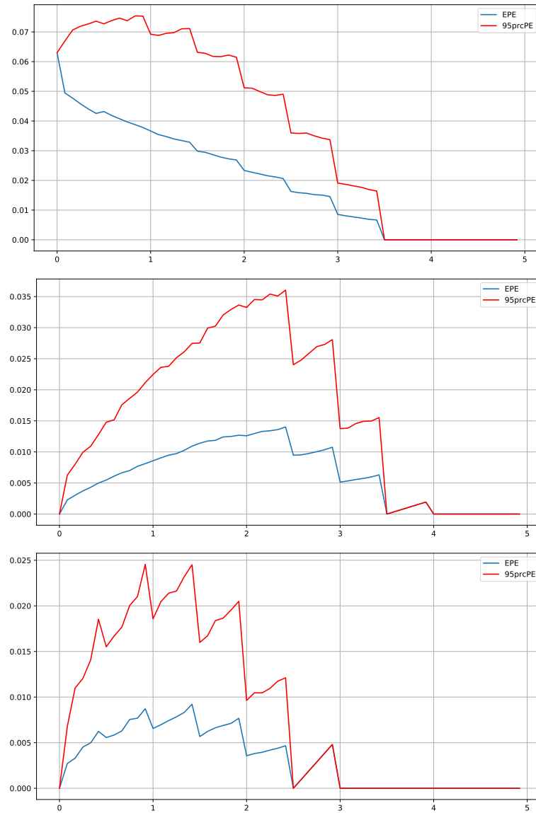
Figure 5: Expected exposure and quantile potential future exposure profiles for three different IRS contracts
