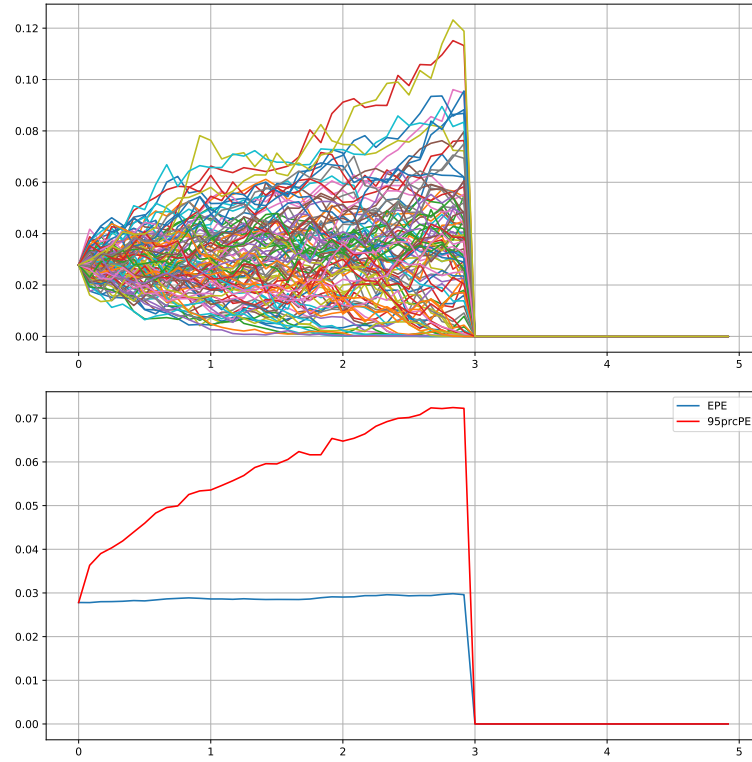
Receiver swaption fixed 0.044 2Y IRS in 3Y expiry time, cash equivalent settlement. All notionals are equal 1. Sample paths (upper pane) and EE profiles (lower pane).
