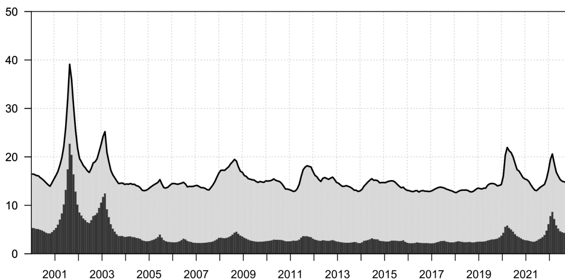
Figure 4: The dynamic connectedness between uncertainty measures – the total spillover index
